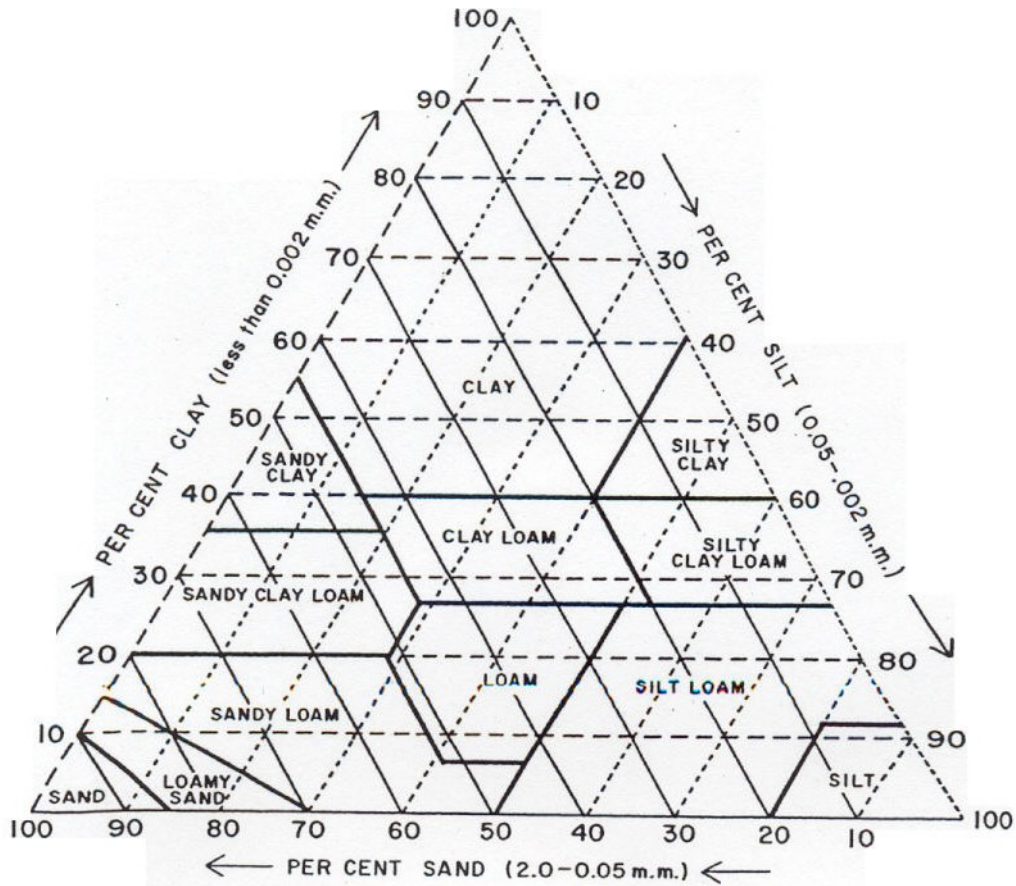
THE TEXTURAL TRIANGLE, SHOWING THE COMMON SOIL CLASSES
